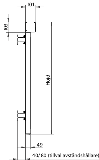
Skruvskena (standard)
